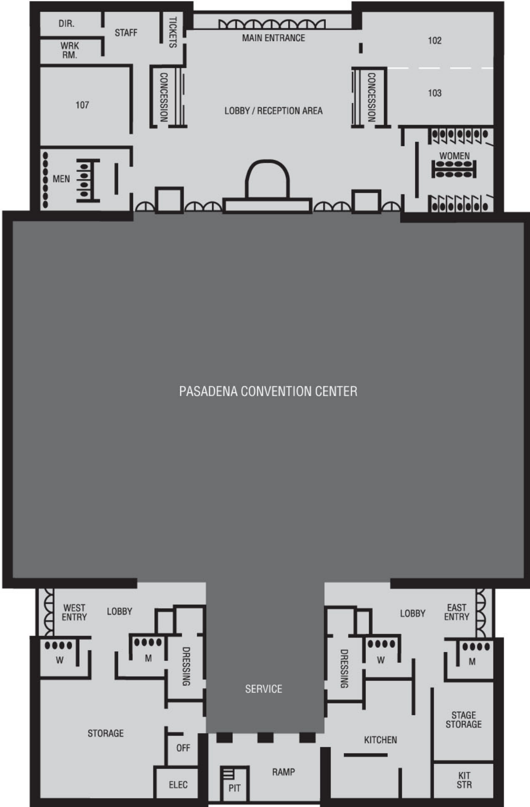
CONVENTION CENTER ALTERNATE CONFIGURATIONS
